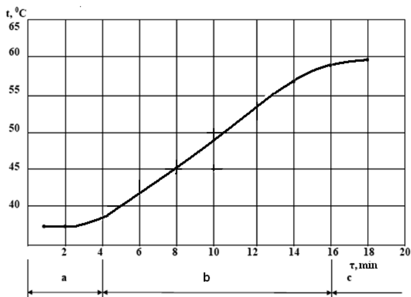
Fig. 4. Dependence of temperature change of oil in vessel on time
