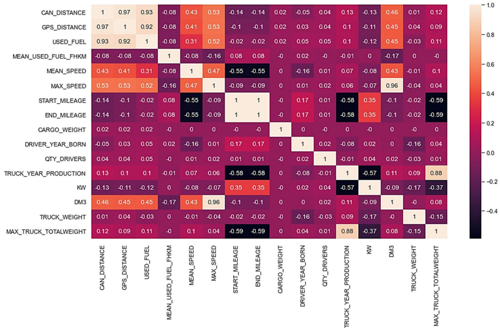
Fig. 3. Matrix of correlation of numerical features
