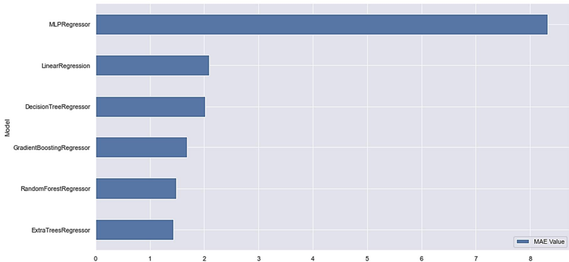
Fig. 4. Models comparison
